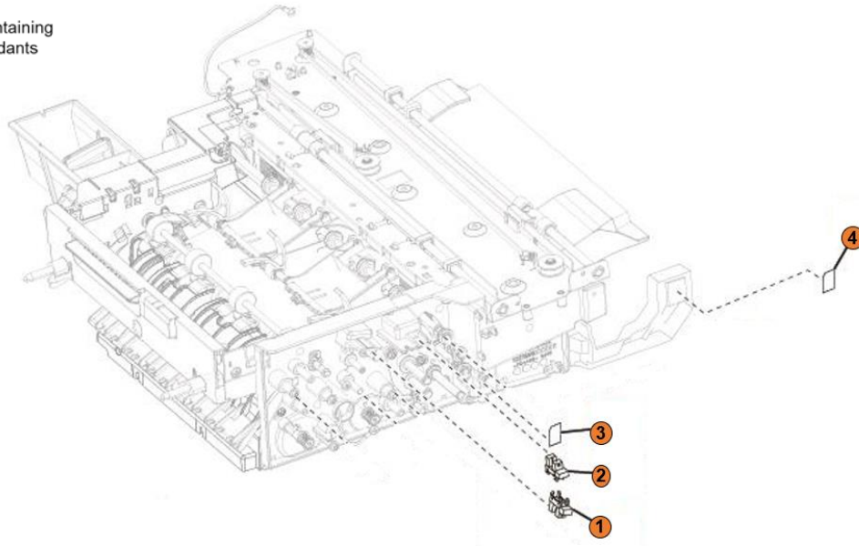
Figure 31.1: Paper Handling Options– Staple Finisher Front
