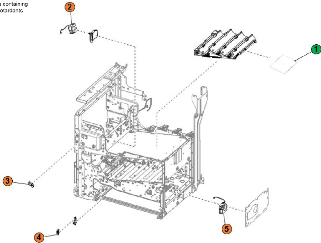
Figure 18.1: Electronics - front
